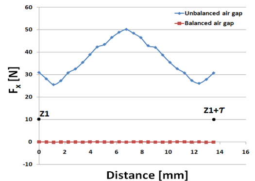
Figure 12. Normal attractive force by moving armature core.
