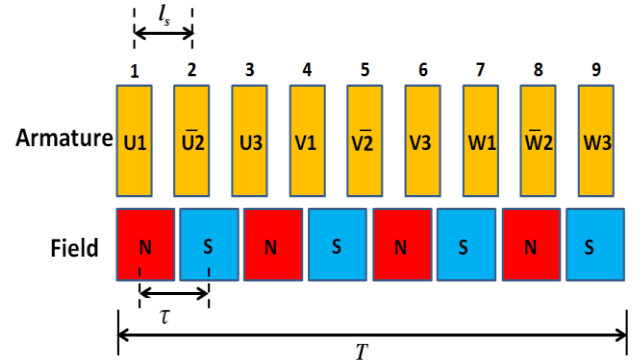
Figure 9. Configuration of nine armature cores and eight field magnets.
