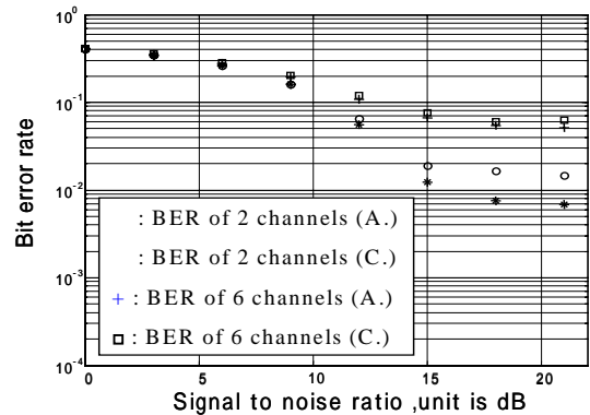
Fig. 5 : BER under interference environment
